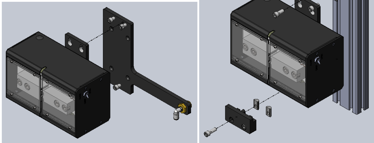
Figure 21. Stretch Grips Installation
